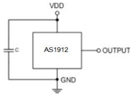
Figure 1, Typical Application Circuit of AS1912
