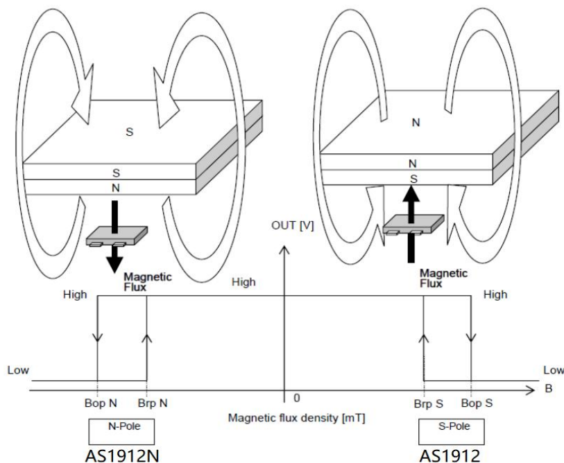
Fig 4, Magnetic Operation Characteristic of AS1912 or AS1912N
